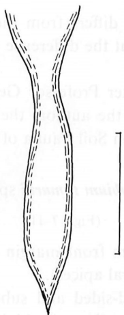
Fig. 6. Apical part of fused paramere of Lathrobium imadatei sp. nov. (paratype). Scale: 0.5 mm.
